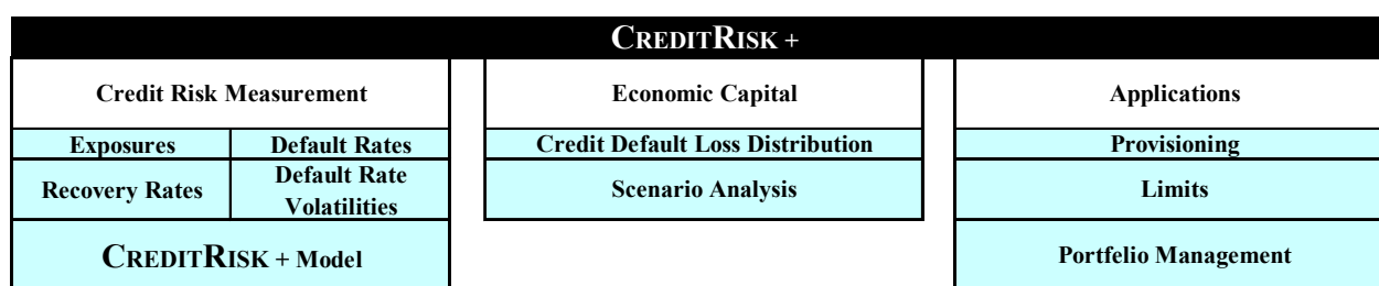
Figure 1. CreditRisk+ System
